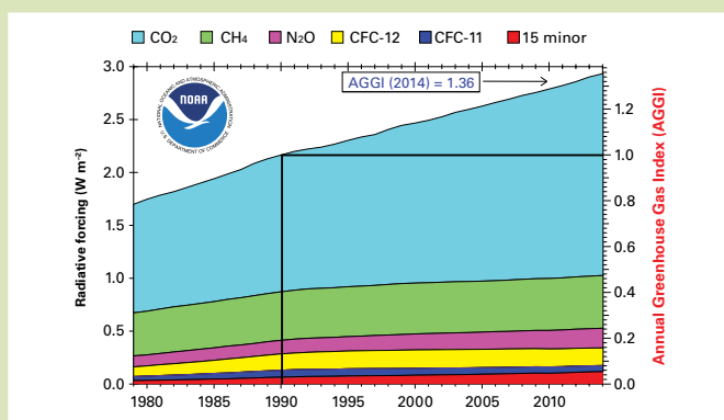
Figure 1. Atmospheric radiative forcing, relative to 1750, of LLGHGs and the 2014 update of the NOAA Annual Greenhouse Gas Index (AGGI)
